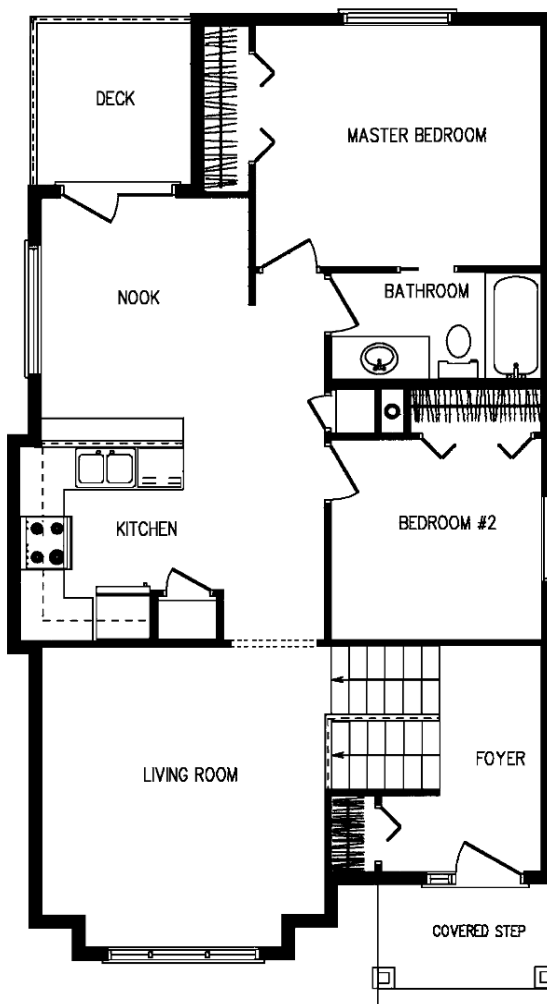
MAIN FLOOR PLAN 965 SQUARE FEET
